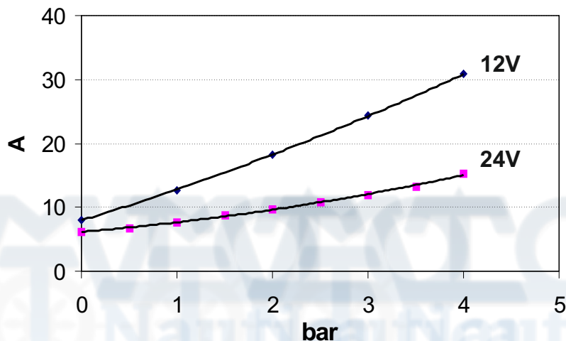
DIAGRAMMA ASSORBIMENTI (acqua) AMPERE-DRAW DIAGRAM (water)
