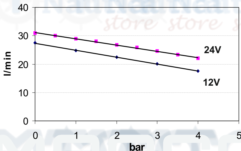
DIAGRAMMA PORTATA (acqua) FLOW RATES DIAGRAM (water)
